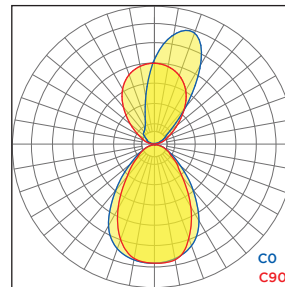
Asymmetric Indirect Micro Prismatic Direct
